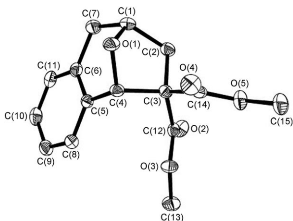
Figure 2. ORTEP drawing for the product 2a . The thermal ellipsoids drawn at the 30% probability level.
